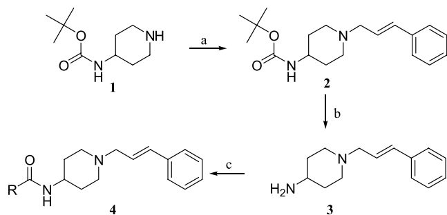
Scheme 1. Reagents and conditions: (a) cinnamyl chloride, K_2CO_3 , DMF, 50 °C, 76%; (b) 4 N HCl/dioxane, 25 °C, 4 h, quantitative; (c) RCOOH , PS-DCC, ^8 HOBt, DMF, 25 °C.
